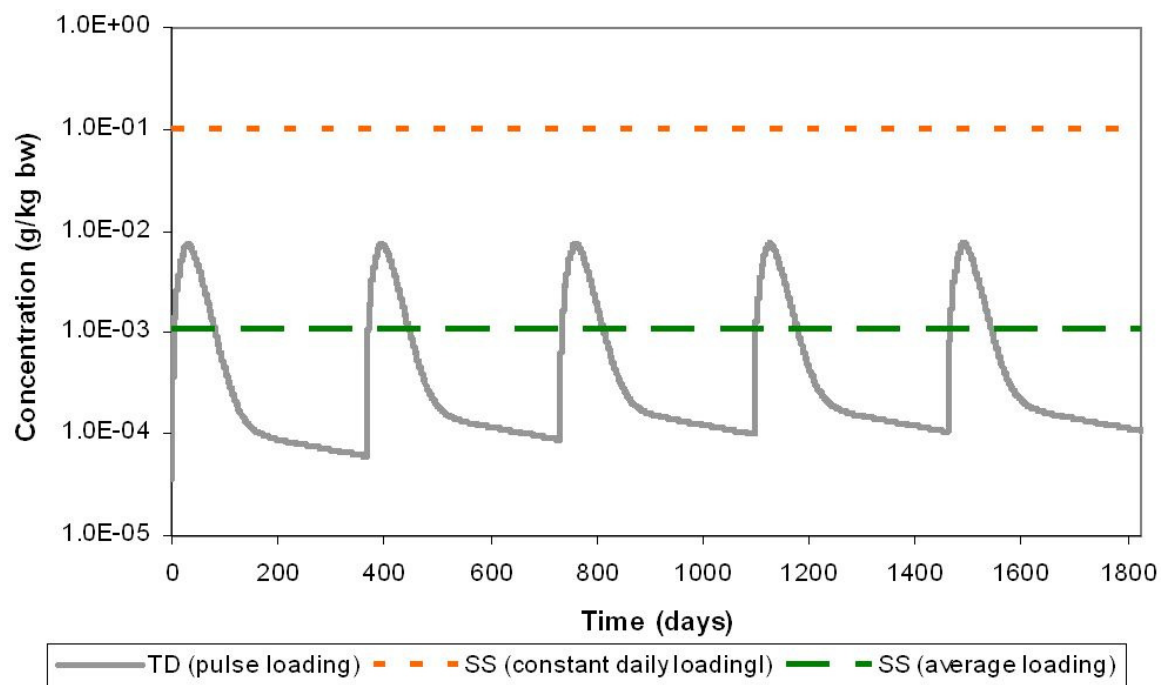
Figure 4-27 Comparison between steady-state and time-dependent bioaccumulation model predictions of metaflumizone concentrations in forage fish B. TD (pulse loading) represents time-dependent model predictions with application rate of 14g/application at 7-day intervals; SS(constant daily loading) represents steady-state model predictions with daily loading of 14g of metaflumizone; SS(average loading) represents steady-state model predictions with daily loading of 0.1534g of metaflumizone.
