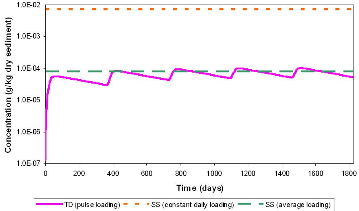
Figure 4-22 Comparison between steady-state and time-dependent bioaccumulation model predictions of metaflumizone concentrations in sediment. TD (pulse loading) represents time-dependent model predictions with application rate of 14g/application at 7-day intervals; SS(constant daily loading) represents steady-state model predictions with daily loading of 14g of metaflumizone; SS(average loading) represents steady-state model predictions with daily loading of 0.1534g of metaflumizone.
