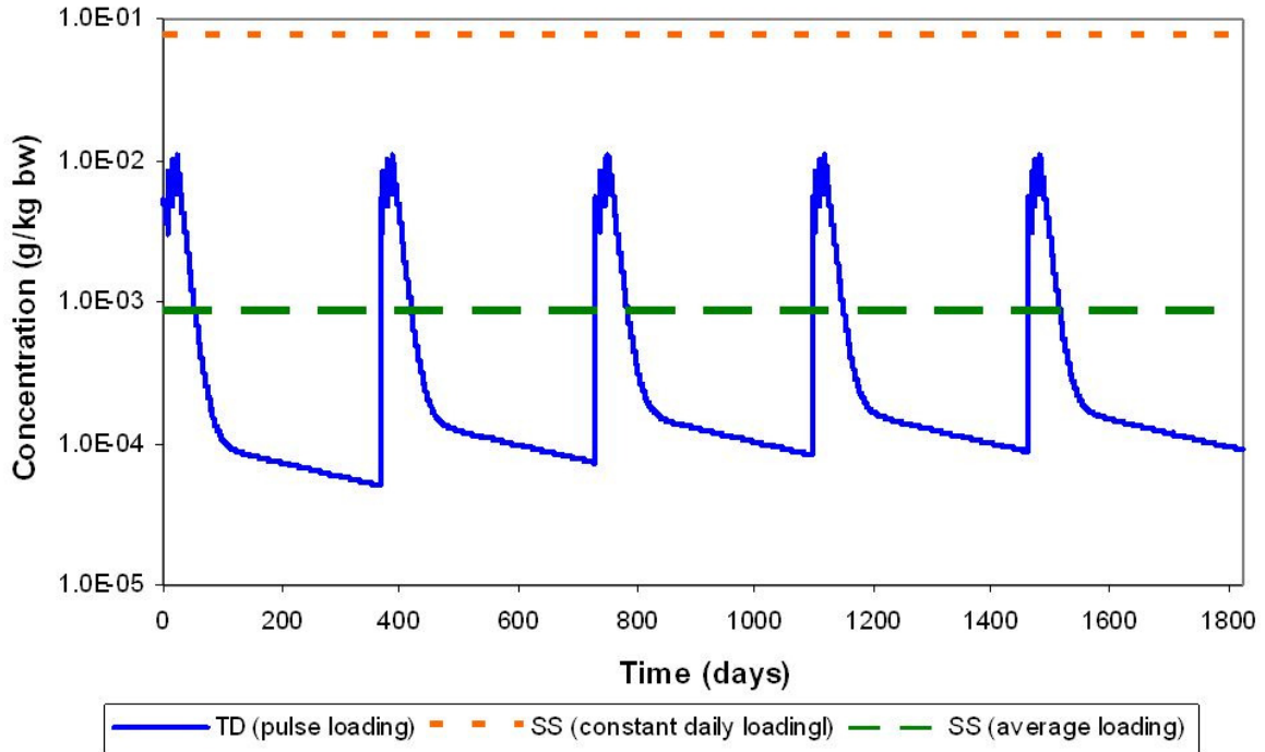
Figure 4-23 Comparison between steady-state and time-dependent bioaccumulation model predictions of metaflumizone concentrations in phytoplankton. TD (pulse loading) represents time-dependent model predictions with application rate of 14g/application at 7-day intervals; SS(constant daily loading) represents steady-state model predictions with daily loading of 14g of metaflumizone; SS(average loading) represents steady-state model predictions with daily loading of 0.1534g of metaflumizone.
