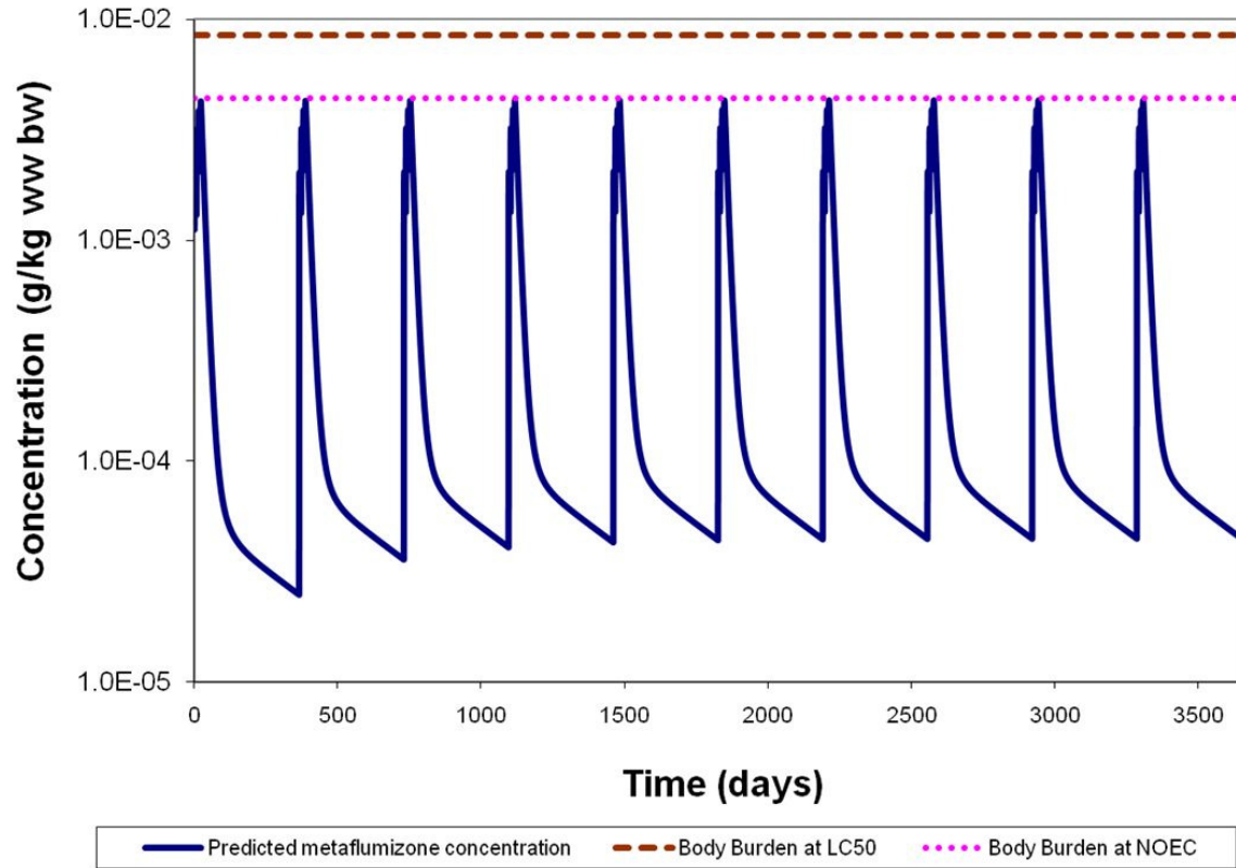
Figure 4-17 Comparison between the predicted metaflumizone concentration in chironormus tentans and the calculated internal body burden of metaflumizone in chironormus tentans associated with the LC50 and NOEC for survival and reproduction
