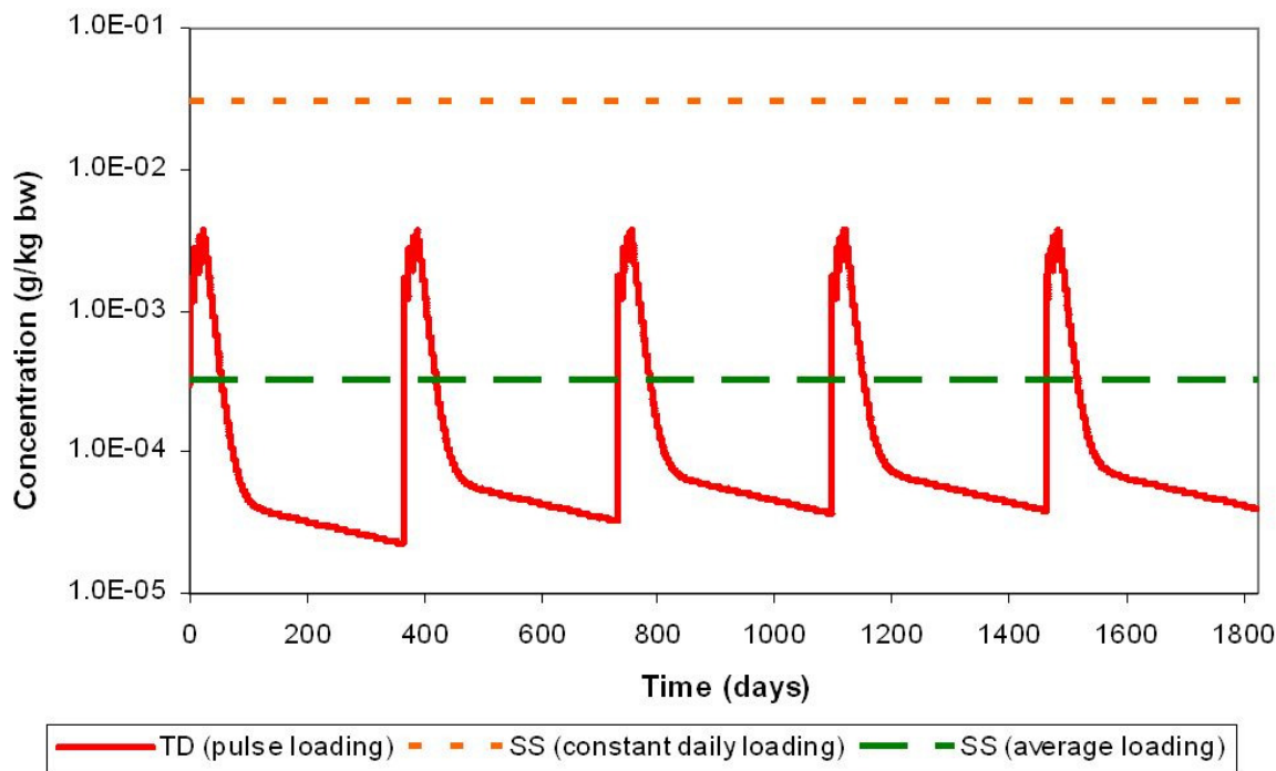
Figure 4-25 Comparison between steady-state and time-dependent bioaccumulation model predictions of metaflumizone concentrations in diporeia. TD (pulse loading) represents time-dependent model predictions with application rate of 14g/application at 7-day intervals; SS(constant daily loading) represents steady-state model predictions with daily loading of 14g of metaflumizone; SS(average loading) represents steady-state model predictions with daily loading of 0.1534g of metaflumizone.
