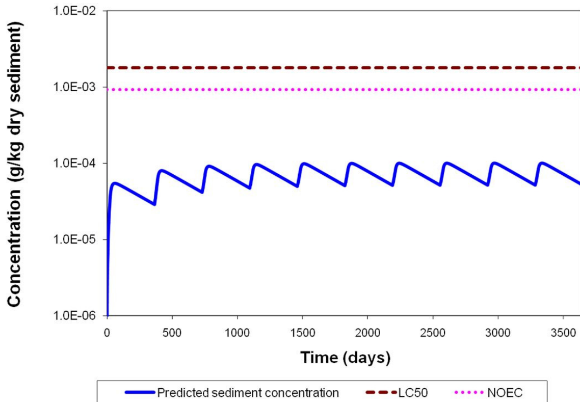
Figure 4-15 Comparison between the predicted metaflumizone concentration in sediment to the LC50 and NOEC of metaflumizone in Chironomus tentans (g/kg dry weight)
