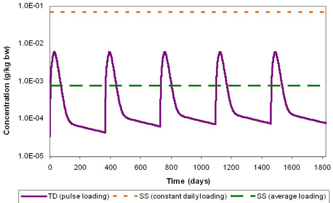
Figure 4-26 Comparison between steady-state and time-dependent bioaccumulation model predictions of metaflumizone concentrations in forage fish A. TD (pulse loading) represents time-dependent model predictions with application rate of 14g/application at 7-day intervals; SS(constant daily loading) represents steady-state model predictions with daily loading of 14g of metaflumizone; SS(average loading) represents steady-state model predictions with daily loading of 0.1534g of metaflumizone.
