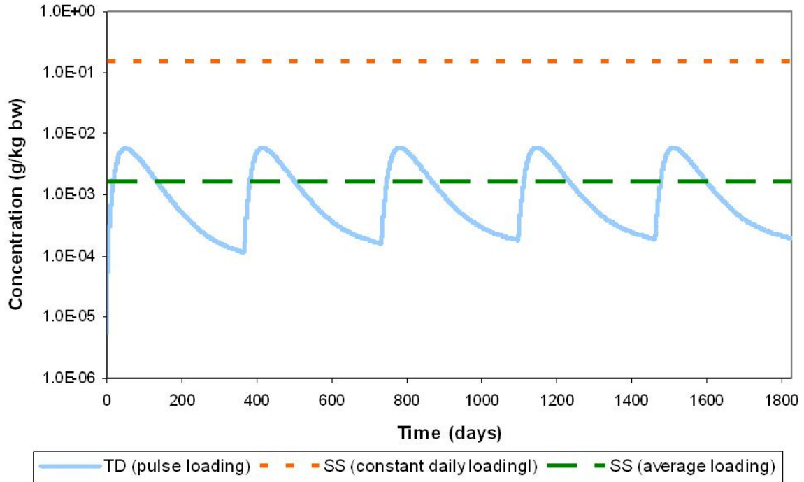
Figure 4-28 Comparison between steady-state and time-dependent bioaccumulation model predictions of metaflumizone concentrations in piscivorous fish. TD (pulse loading) represents time-dependent model predictions with application rate of 14g/application at 7-day intervals; SS(constant daily loading) represents steady-state model predictions with daily loading of 14g of metaflumizone; SS(average loading) represents steady-state model predictions with daily loading of 0.1534g of metaflumizone.
