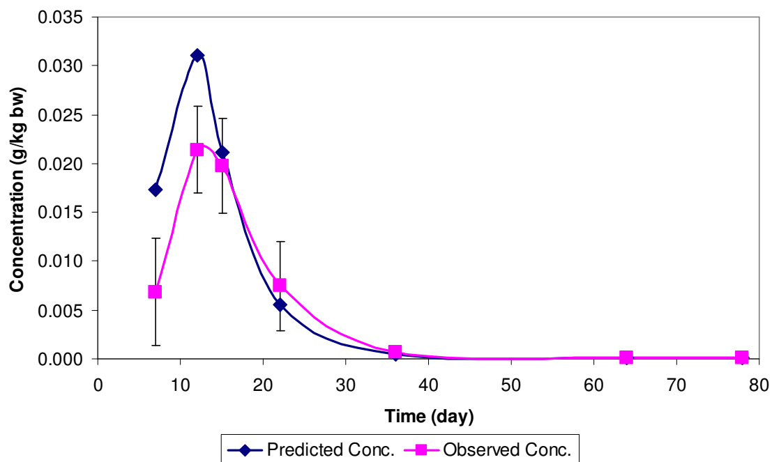
Figure 4-14 Model predicted and the mean of the observed metaflumizone concentrations (g/kg body weight) in fish. Error bars represent one standard deviation of the mean metaflumizone concentration. (n = 3)
