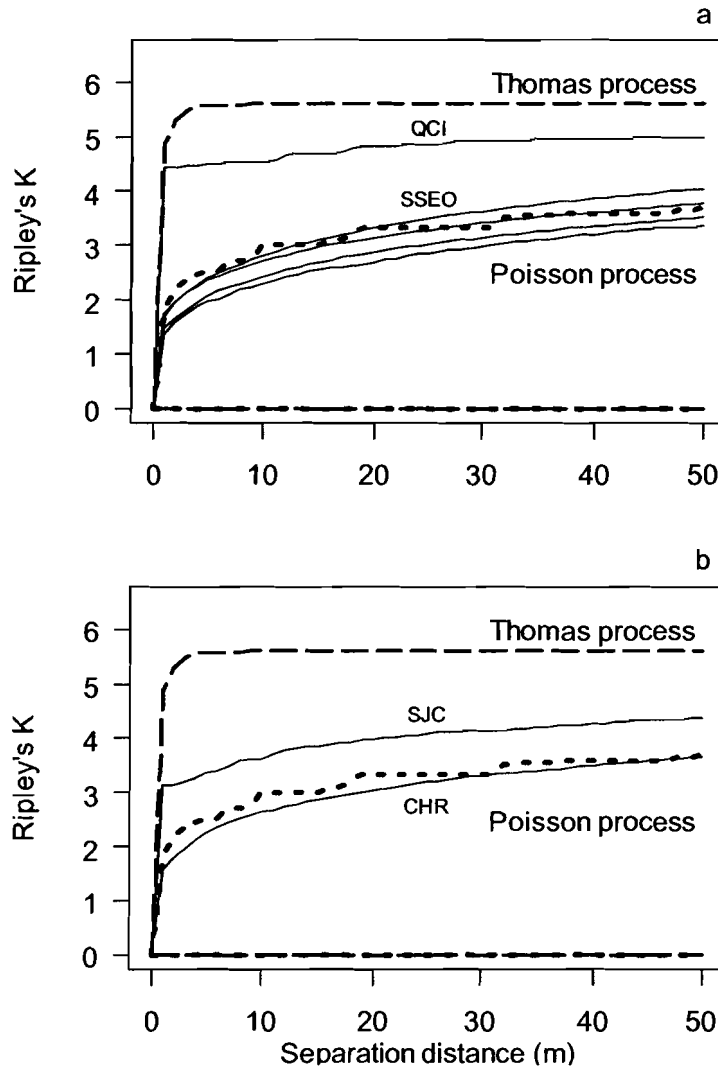
Figure 12 The empirical K -functions for ROV data simulated from spatial models compared to the empirical K -functions from the actual underwater visual survey data: a. submersible data and b. ROV data. The empirical K -functions for the real survey data are shown by thin solid lines: Queen Charlotte Islands (QCI), Southern Southeast Outside (SSEO), San Juan Channel (SJC), and Chiswell Ridge (CHR). The submersible surveys for the remainder of the Southeast Outside sites are shown by not labelled (NSEO, CSEO, and EYKT). The dashed and dotted lines represent the upper confidence envelope of the empirical K -functions for the simulated data from the Thomas process and Poisson process, respectively. The lower confidence envelope for both processes was a horizontal line at Ripley's K equal to 0.
