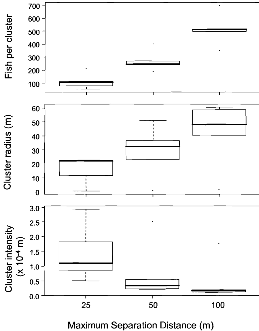
Figure 11 The effect of the maximum separation distance used in the parameter estimation procedure ( h_r ) on Thomas process parameter estimates: fish per cluster ( \mu ), cluster radius ( \rho ), and cluster intensity ( \lambda ). The baseline value used was h_r = 50 . The boxplots show the distribution of parameter values for the five sites surveyed with manned submersibles.
