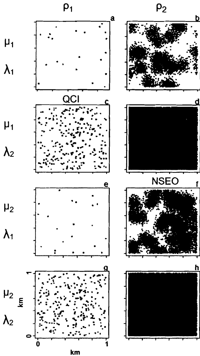
Figure 3 Simulated spatial distributions of rockfish within 1-km 2 survey areas based on the estimated Thomas process parameters, where \mu_1 = 247 , \mu_2 = 399 , \rho_1 = 0.8 , \rho_2 = 51 , \lambda_1 = 2.2 \times 10^{-5} , \lambda_2 = 2.4 \times 10^{-5} ). Simulations represent the extreme values for all sites. Patterns typical of the Queen Charlotte Islands, BC ( \mu_1, \rho_1, \lambda_2 ) and NSEO within the Southeast Outside District, AK ( \mu_2, \rho_2, \lambda_1 ) are labeled above the representative plot. Points represent individual fish.
