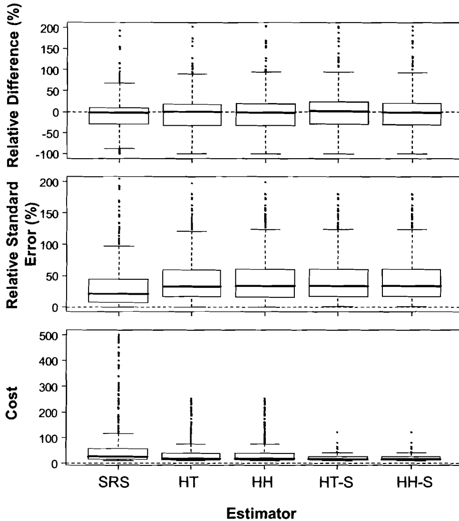
Figure 4 The performance of the five sampling protocols under the clustered rockfish model. Performance measures include: relative difference (%), relative standard error (%), and cost. The Sampling protocols used were: simple random sampling (SRS), adaptive cluster sampling with Horvitz-Thompson estimator (HT), adaptive cluster sampling with Hansen-Hurwitz estimator (HH), adaptive cluster sampling with stopping rule and Horvitz-Thompson estimator (HT-s), and adaptive cluster sampling with stopping rule and Hansen-Hurwitz estimator (HH-s). Outliers are more than 1.5 times the distance of the inter-quartile range.
