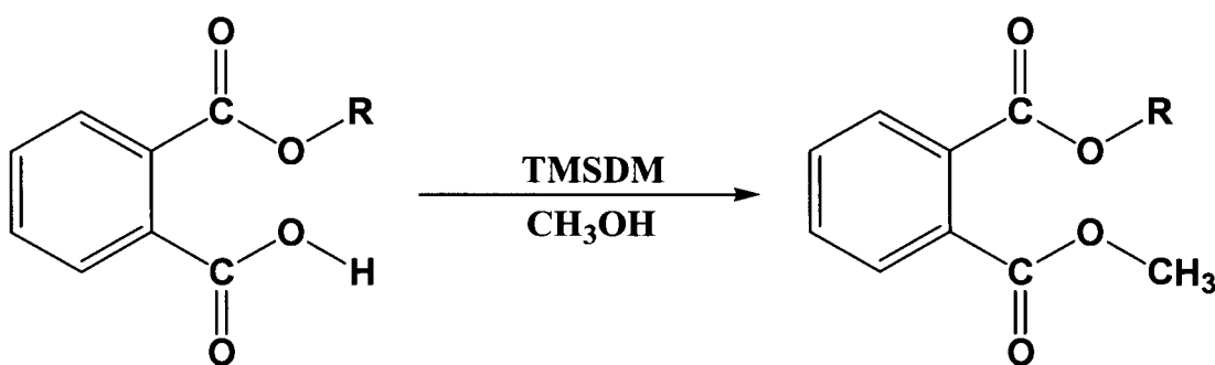
Figure 10: Methylation of monophthalate esters.
