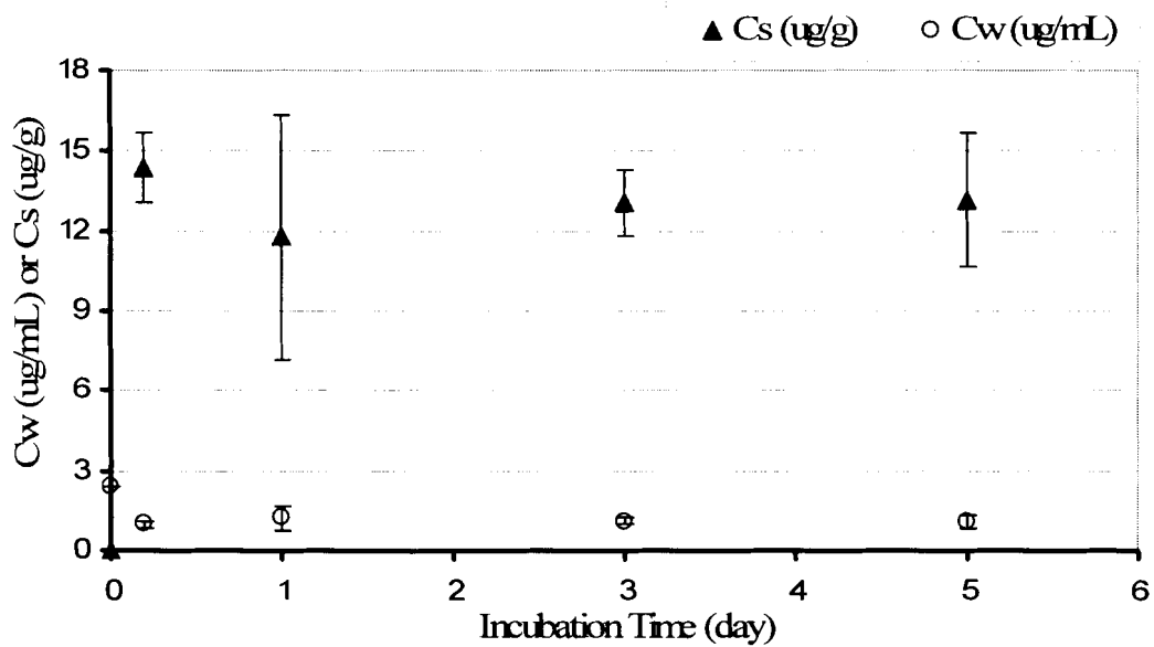
Figure 33: Sorption curve for MC10 on fresh water sediment. Water and sediment concentrations for each time point are mean of 3 values (n=3), error bars are 2 standard deviations. Sediment uptake rate constant ( k_{sw} ) and water elimination rate constant ( k_{ws} ) are estimated to be 17.8 and 1.47 respectively (non-linear regression using equation 14).
