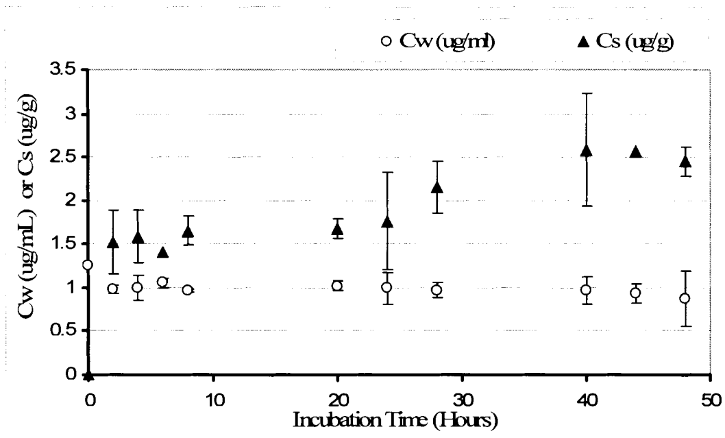
Figure 23: Sorption curve for MnOP on marine water sediment. Water and sediment concentrations for each time point are mean of 3 values (n=3), error bars are 2 standard deviations. Sediment reached equilibrium within 24 h and there is no significant difference (p=0.38 at 95%, one-way ANOVA) in sediment concentration from day 1 to till the end of the incubation period.
