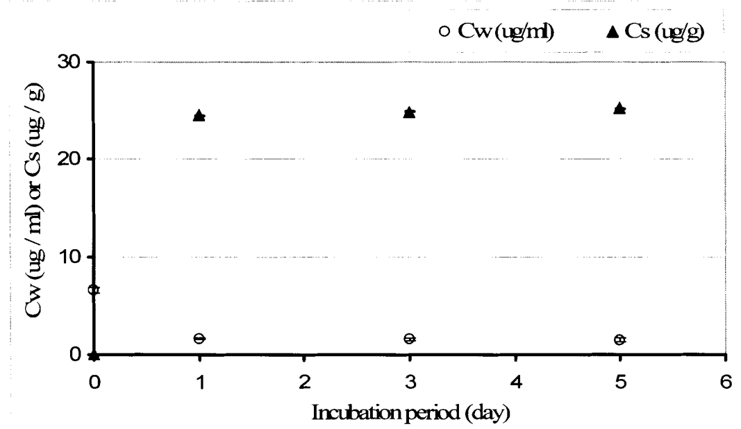
Figure 22: Sorption curve for MEP on marine water sediment. Water and sediment concentrations for each time point are mean of 3 values ( n=3 ), error bars are 2 standard deviations. Sediment reached equilibrium within 24 h and there is no significant difference ( p=0.57 at 95%, one-way ANOVA) in sediment concentration from day 1 to till the end of the incubation period.
