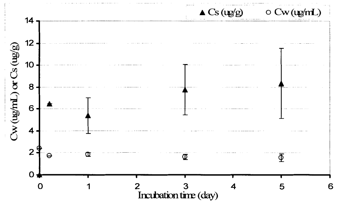
Figure 32: Sorption curve for MC9 on fresh water sediment. Water and sediment concentrations for each time point are mean of 3 values ( n=3 ), error bars are 2 standard deviations. Sediment uptake rate constant ( k_{sw} ) and water elimination rate constant ( k_{ws} ) are estimated to be 5.98 and 1.39 respectively (non-linear regression using equation 14).
