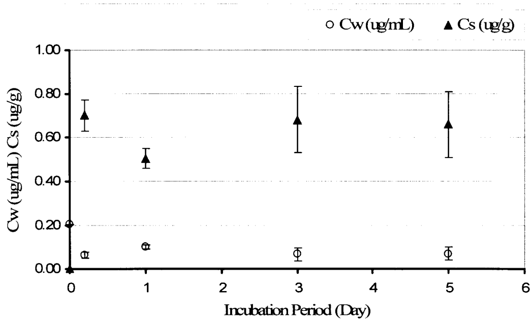
Figure 19: Sorption curve for MC7 on marine water sediment. Water and sediment concentrations for each time point are mean of 3 values (n=3), error bars are 2 standard deviations. Sediment uptake rate constant ( k_{SW} ) and water elimination rate constant ( k_{WS} ) are estimated to be 6.05 and 0.45 respectively (non-linear regression using equation 14).
