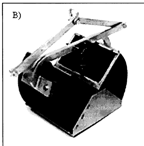
Figure 9: Field sampling equipment: Sediment Grab Sampler (Petit Ponar).
