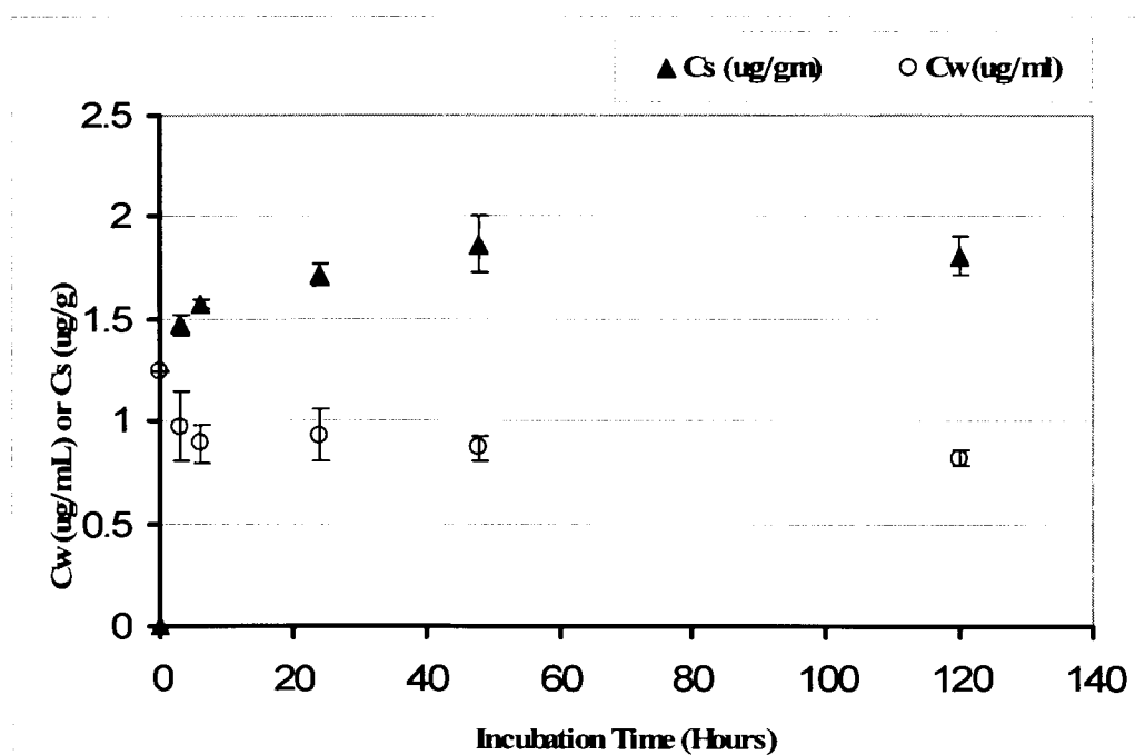
Figure 16: Sorption curve for MEHP on marine water sediment. Water and sediment concentrations for each time point are mean of 3 values (n=3), error bars are 2 standard deviations. Sediment reached an equilibrium within 24 h and there is no significant difference (p=0.33 at 95%, one-way ANOVA) in sediment concentration from day 1 to till the end of the incubation period.
