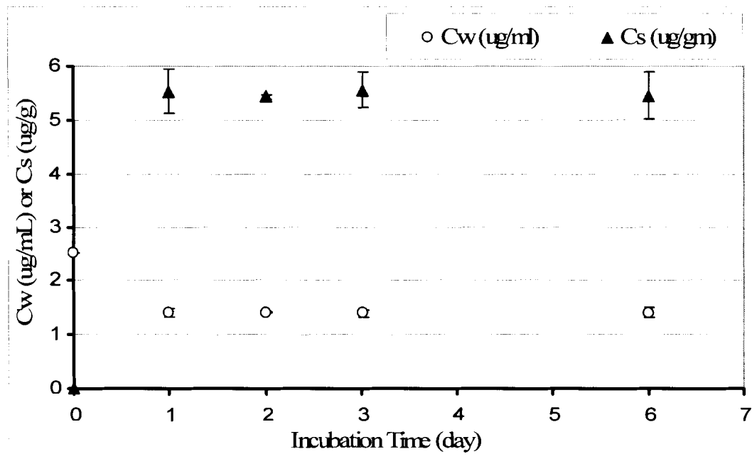
Figure 24: Sorption curve for MBzP on marine water sediment. Water and sediment concentrations for each time point are mean of 3 values (n=3), error bars are 2 standard deviations. Sediment reached equilibrium within 24 h and there is no significant difference (p=0.76 at 95%, one-way ANOVA) in sediment concentration from day 1 to till the end of the incubation period.
