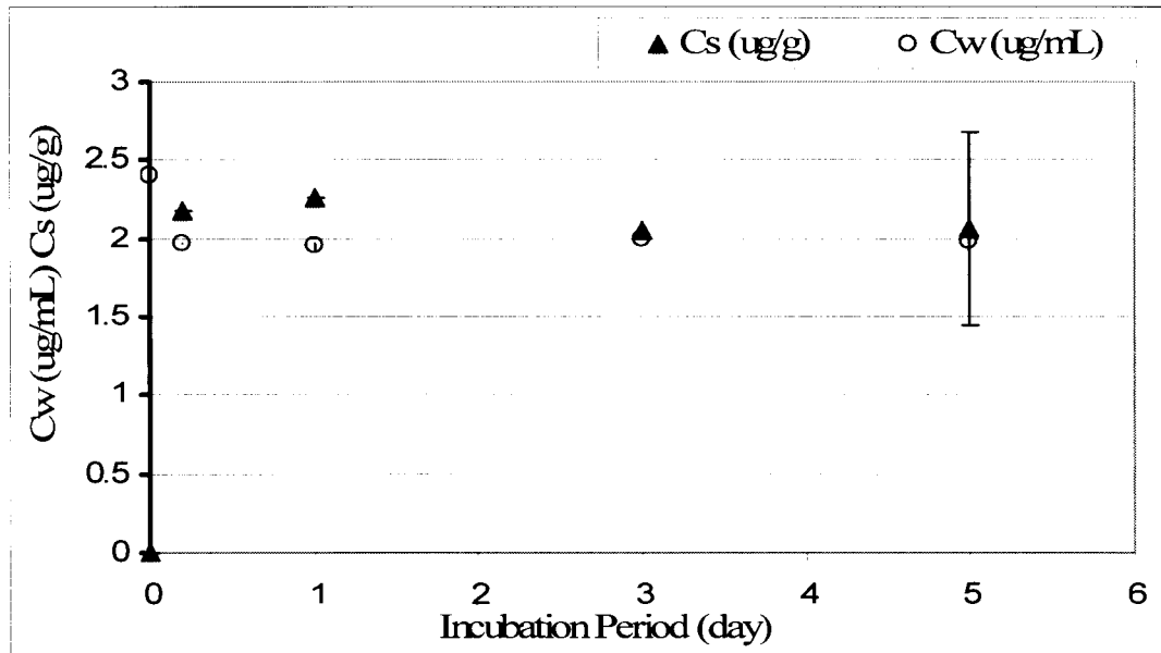
Figure 20: Sorption curve for MC9 on marine water sediment. Water and sediment concentrations for each time point are mean of 3 values (n=3), error bars are 2 standard deviations. Sediment uptake rate constant ( k_{SW} ) and water elimination rate constant ( k_{WS} ) are estimated to be 19.2 and 17.1 respectively (non-linear regression using equation 14).
