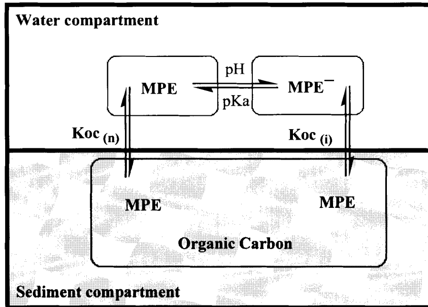
Figure 6: Graphic representation of effect of ionization on the partitioning of a chemical between sediment and water compartments. MPE is neutral form, MPE - is the ionized form, K_{OC(n)} and K_{OC(i)} are the organic carbon partition coefficients for neutral and ionized forms of the MPEs respectively.
