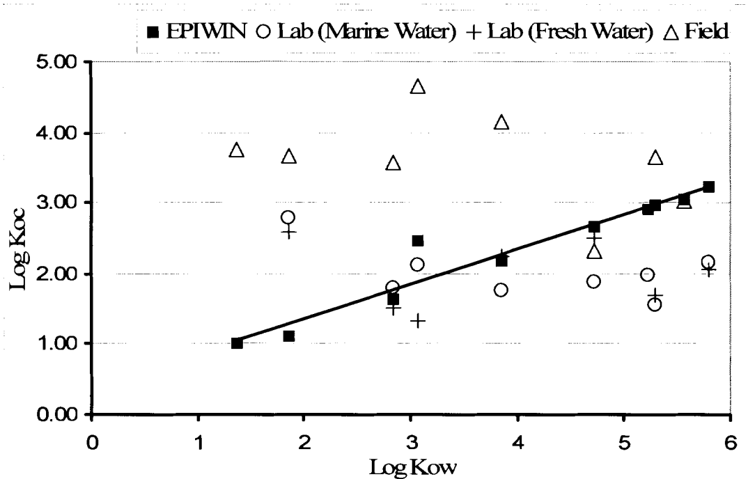
Figure 38: Graph showing Log K OC (EPIWIN calculated Log K OC , Experimental Log K OC (Marine sediment and Fresh water sediment) and Field derived Log K OC values vs Log K ow . Solid line represents regression fit for the predicted values by EPIWIN ( r^2=0.94 ).
