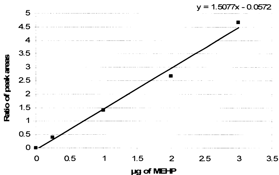
Figure 13: Calibration curve for MEHP with MnOP as internal standard. Solid line represents regression line ( y=1.5077x - 0.0572 ). R^2 = 0.99 .
