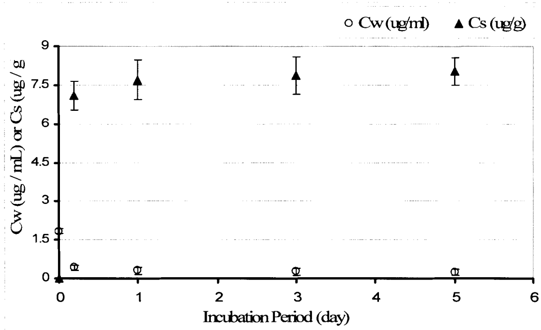
Figure 25: Sorption curve for MEHP on fresh water sediment. Water and sediment concentrations for each time point are mean of 3 values ( n=3 ), error bars are 2 standard deviations. Sediment reached equilibrium within 24 h and there is no significant difference ( p=0.55 at 95%, one-way ANOVA) in sediment concentration from day 1 to till the end of the incubation period.
