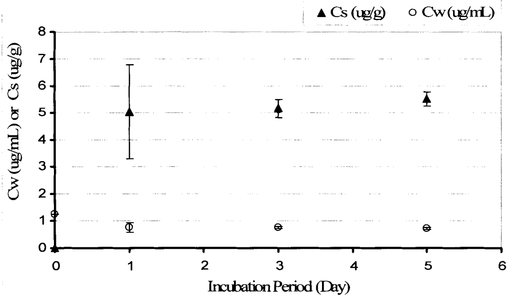
Figure 30: Sorption curve for MnOP on fresh water sediment. Water and sediment concentrations for each time point are mean of 3 values (n=3), error bars are 2 standard deviations. Sediment reached equilibrium within 24 h and there is no significant difference ( p=0.45 at 95%, one-way ANOVA) in sediment concentration from day 1 to till the end of the incubation period.
