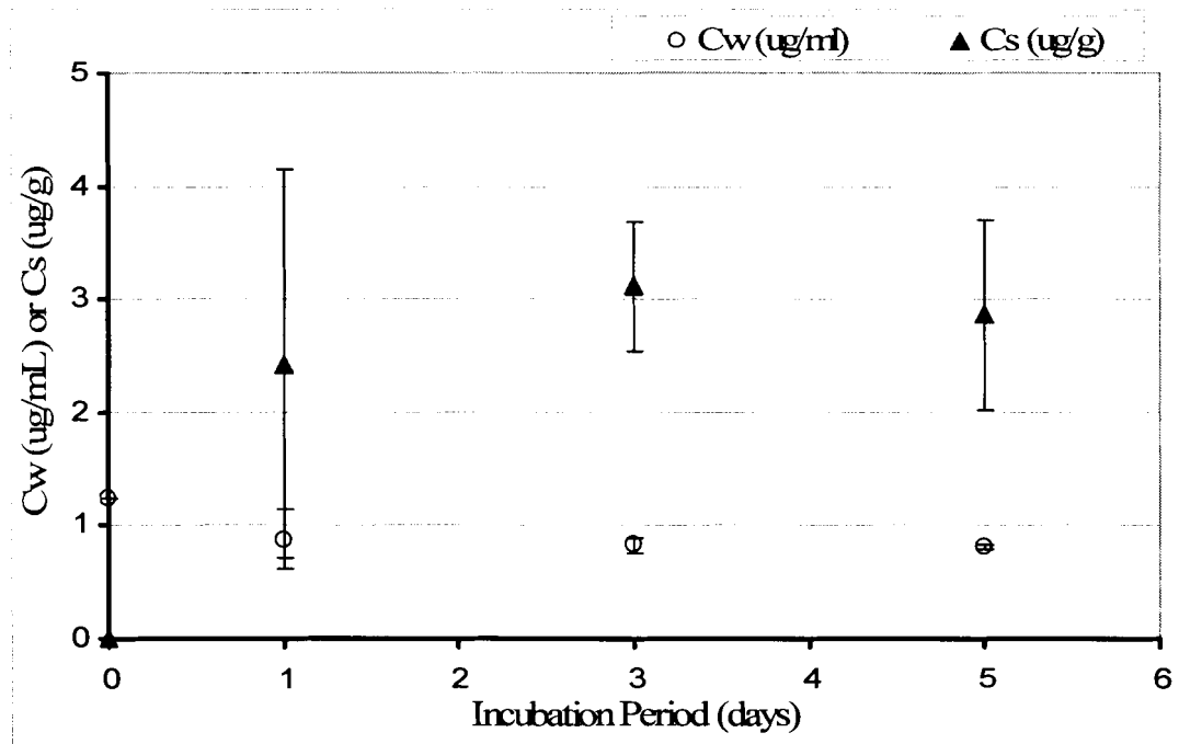
Figure 27: Sorption curve for MBuP on fresh water sediment. Water and sediment concentrations for each time point are mean of 3 values (n=3), error bars are 2 standard deviations. Sediment reached equilibrium within 24 h and there is no significant difference (p=0.40 at 95%, one-way ANOVA) in sediment concentration from day 1 to till the end of the incubation period.
