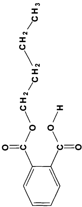
Mono-n-butyl Phthalate (MnBP)
