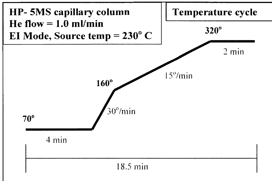
Figure 11: Temperature cycle program in GC for MPE derivative analysis.
