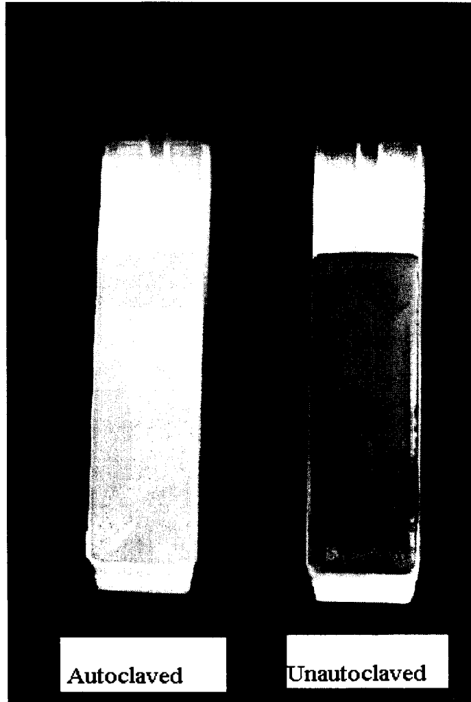
Figure 14: Easicult plates (autoclaved (left) and unautoclaved (right) sediment inoculations).
