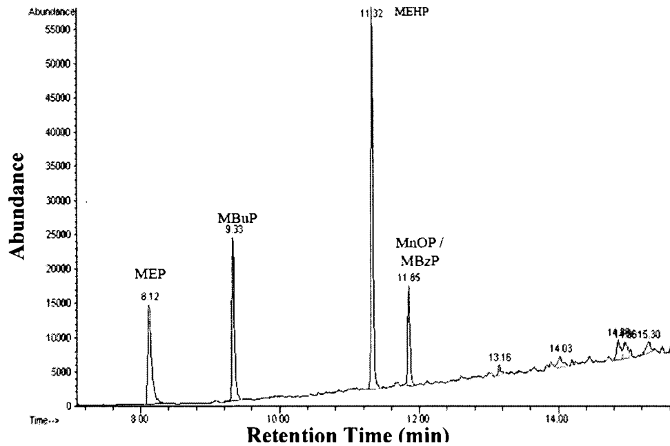
Figure 12: Chromatogram showing peaks, retention time, and abundance for MEP, MBuP, MEHP, MnOP and MBzP.
