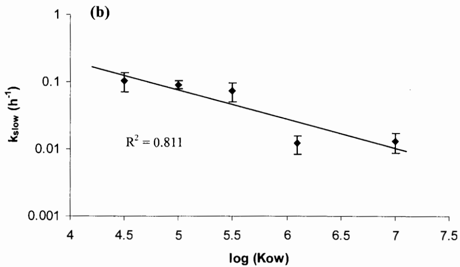
Figure 3-6 Estimated slow uptake rate constants ( h^{-1} ), \pm 1 standard error, versus \log Kow for chemicals in the Port Moody sediment aged for (a) 21 days and for (b) 102 days
