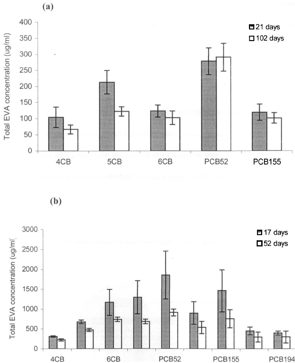
Figure 3-10 Equilibrium concentrations in EVA ( \mu\text{g}/\text{mL} ) for chemicals in (a) Port Moody sediment, aged 21 and 102 days, and (b) Robert's Bank sediment, aged 17 and 52 days (error bars represent 95% confidence intervals)
