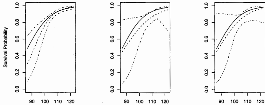
Figure 3.7: Estimated survival curves for the second simulation using the three estimation methods: full data MLE's (left), MCEM (centre), and Bayesian approach (right). The solid line in each plot shows the actual survival curve and the dashed line the estimated curve. The dot-dash lines in the figures give the 95% confidence/credible intervals for the value of \phi(z) for each z in the range of observed values.
