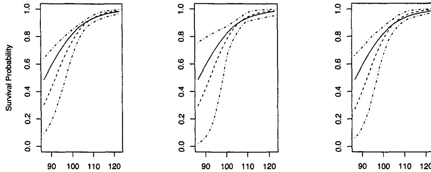
Figure 3.3: Estimated survival curves for the first simulation using the three estimation methods: full data MLE's (left), MCEM (centre), and Bayesian approach (right). The solid line in each plot shows the actual survival curve and the dashed line the estimated curve. The dot-dash lines in the figures give the 95% confidence/credible intervals for the value of \phi(z) . The observed range of covariate values was 86.5 \leq z \leq 122.7 .
