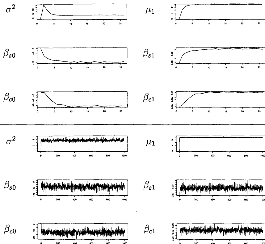
Figure 3.2: Trace plots of the estimates of selected model parameters for each iteration of the MCEM (top) and the Bayesian MH algorithm (bottom) from the first simulation.
