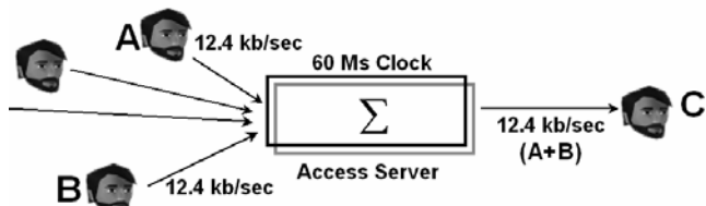
Figure 2. Multi-point, full duplex voice codec with additive bridging where the server can add compressed streams.
