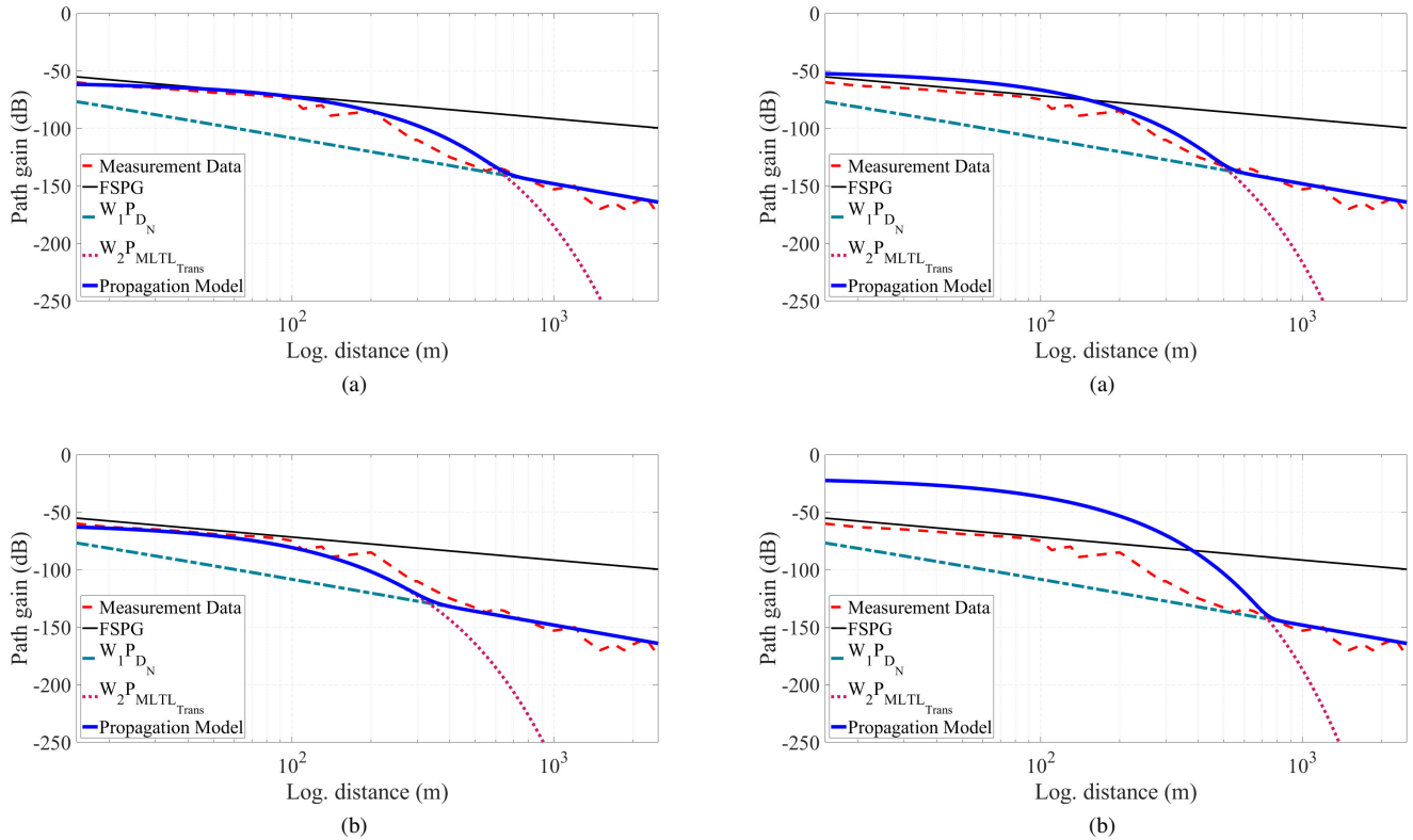
Fig. 8: Comparison between the measured path gain in [23] and our propagation model for r = 1.5\text{m} ( N = 1720 ), W_2 = 1 - W_1 = -70\text{dB} : (a) \epsilon'' = 0.006 and (b) \epsilon'' = 0.01 . The distance scale is logarithmic. The free space path gain (FSPG), W_1 P_{D_N} , and W_2 P_{MLTL_{Trans}} are also plotted to show the dominant parameters.
