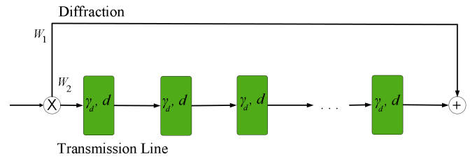
Fig. 1: Through-forest propagation model. The transmission line, in parallel and uncoupled with the diffraction path.
