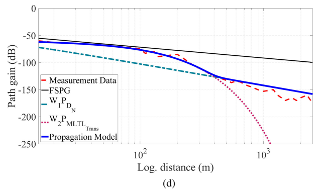
Fig. 7: Comparison between the measured path gain in [23] and our propagation model for \epsilon'' = 0.008 , W_2 = 1 - W_1 = -70\text{dB} : (a) r = 1\text{m} ( N = 2580 ), (b) r = 1.5\text{m} ( N = 1720 ), (c) r = 2\text{m} ( N = 1290 ) and (d) r = 3\text{m} ( N = 860 ). Note that for different r , N is different, and the distance scale is logarithmic. The free space path gain (FSPG), W_1 P_{D_N} , and W_2 P_{MLTL_{Trans}} are also plotted to show the dominant parameters.
