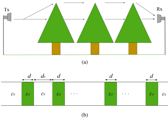
Fig. 2: (a) A depiction of trees between a transmitter and receiver antenna. (b) Two-dimensional multi-layer configuration of in-line trees. The constant thickness of the trees and the free space distance between them are denoted by d and d_0 , respectively. The diffraction and vegetation penetration mechanisms are considered as independent, a simplifying limitation, but their models are connected, again for simplicity, by the number of lossy transmission line sections (trees) being the same as the number of diffraction edges (tree tops).
