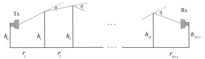
Fig. 4: Geometry for multiple knife-edge diffraction (after [6]).
