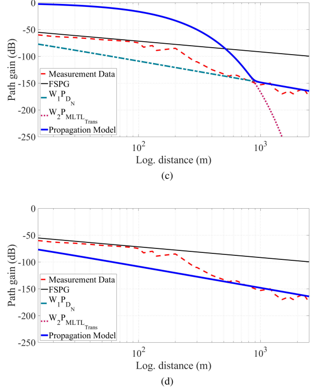
Fig. 9: Comparison between the measured path gain in [23] and our propagation model for \epsilon'' = 0.008 , r = 1.5\text{m} ( N = 1720 ): (a) W_2 = 1 - W_1 = -60\text{dB} , (b) W_2 = 1 - W_1 = -30\text{dB} , (c) W_2 = 1 - W_1 = -1\text{dB} , (d) W_2 = 1 - W_1 = -\infty\text{dB} . The distance scale is logarithmic. The free space path gain (FSPG), W_1 P_{D_N} , and W_2 P_{MLTL_{Trans}} are also plotted to show the dominant parameters.
