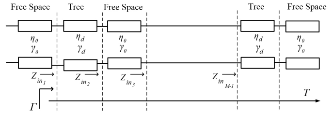
Fig. 3: Equivalent transmission line circuit for the two-dimensional multi-layered configuration of in-line trees (after [34]).
