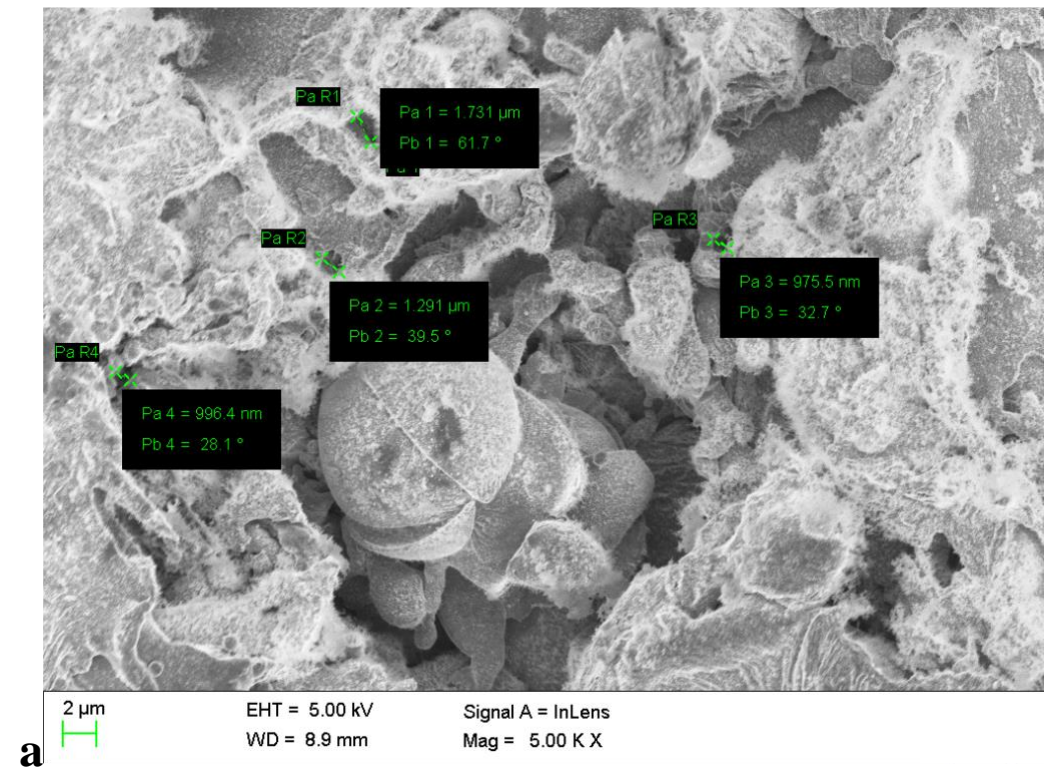
SEM images of wire flame coating at locations (a) and (b)
