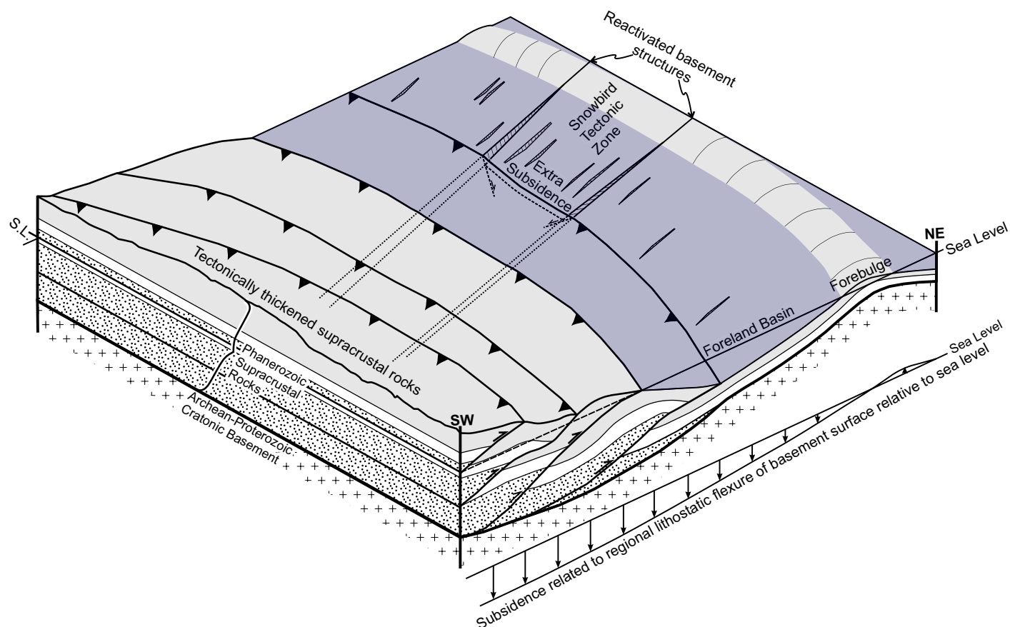
Figure 4. Schematic block diagram showing conceptual model for the formation of the foreland basin by regional lithostatic flexure of the cratonic lithosphere induced by loading of the tectonically thickened supracrustal rocks of the fold-and-thrust belt (modified after Price, 1994, 1973). Also shown is the additional subsidence in the area affected by basement structures that were reactivated as a result of the lithostatic flexure. The forebulge experiences a low rate of subsidence and/or subtle uplift, leading to increased rates of erosion in subaerially exposed sections (Crampton and Allen, 1995; DeCelles and Giles, 1996). The forebulge (and hinge line separating it from the foredeep) represents an area that shifts or migrates over time in response to shortening of the foreland basin with continued subduction (DeCelles and Giles, 1996).
