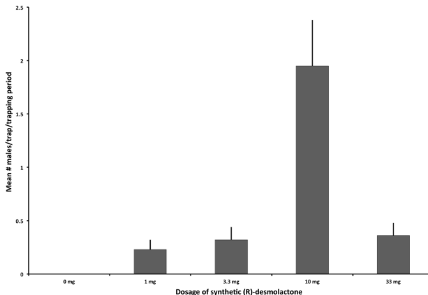
Fig. 5. Captures of male VELB in traps baited with different doses of synthetic (R)-desmolactone (number of beetles captured in 10 mg treatment=43, Friedman's Q=27.31 ). Means with the same letters are not different at P\leq 0.0001 (REGWQ means-separation test [44]).
