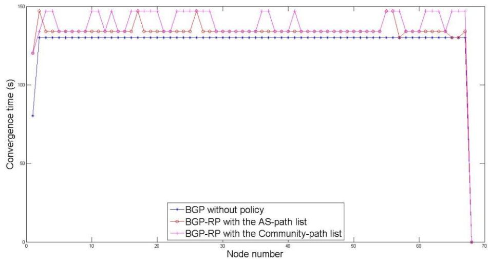
Figure 5.1: Convergence Time for Various Nodes in Network Topology
