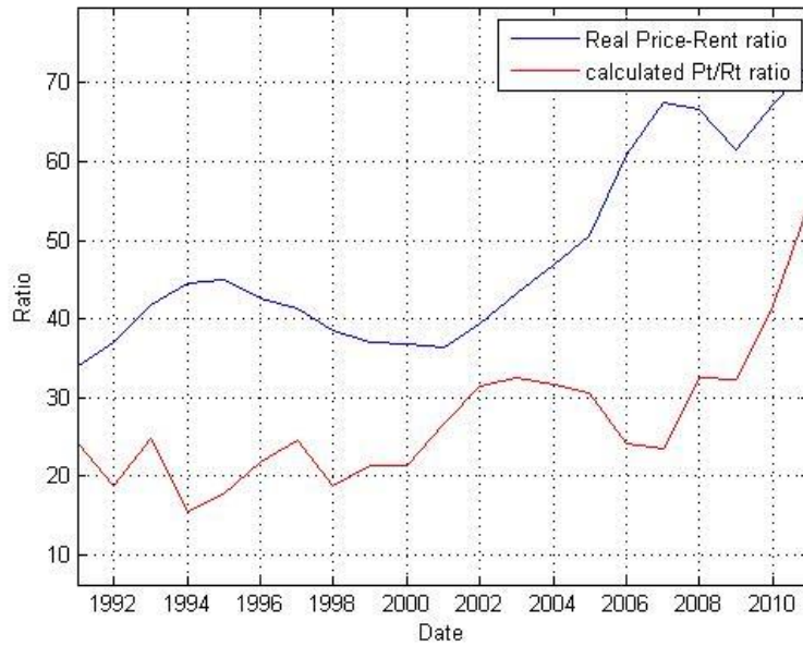
Figure 5(Expected price growth 2%)
