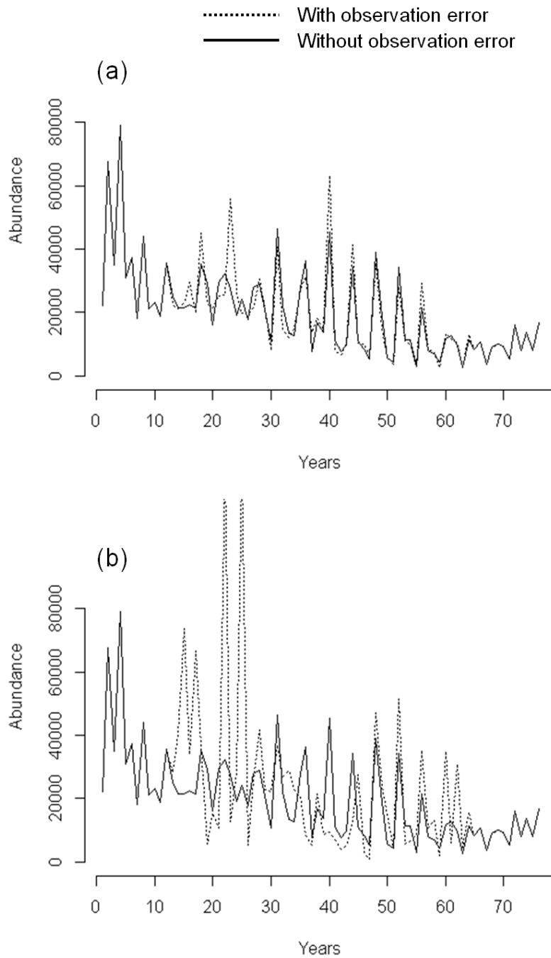
Figure 2: Examples of simulated population abundance produced by the model, with (dotted) and without (solid) observation error at levels of variance of the error term ( \sigma_v^2 ) of 0.05 (a) and 0.5 (b).
