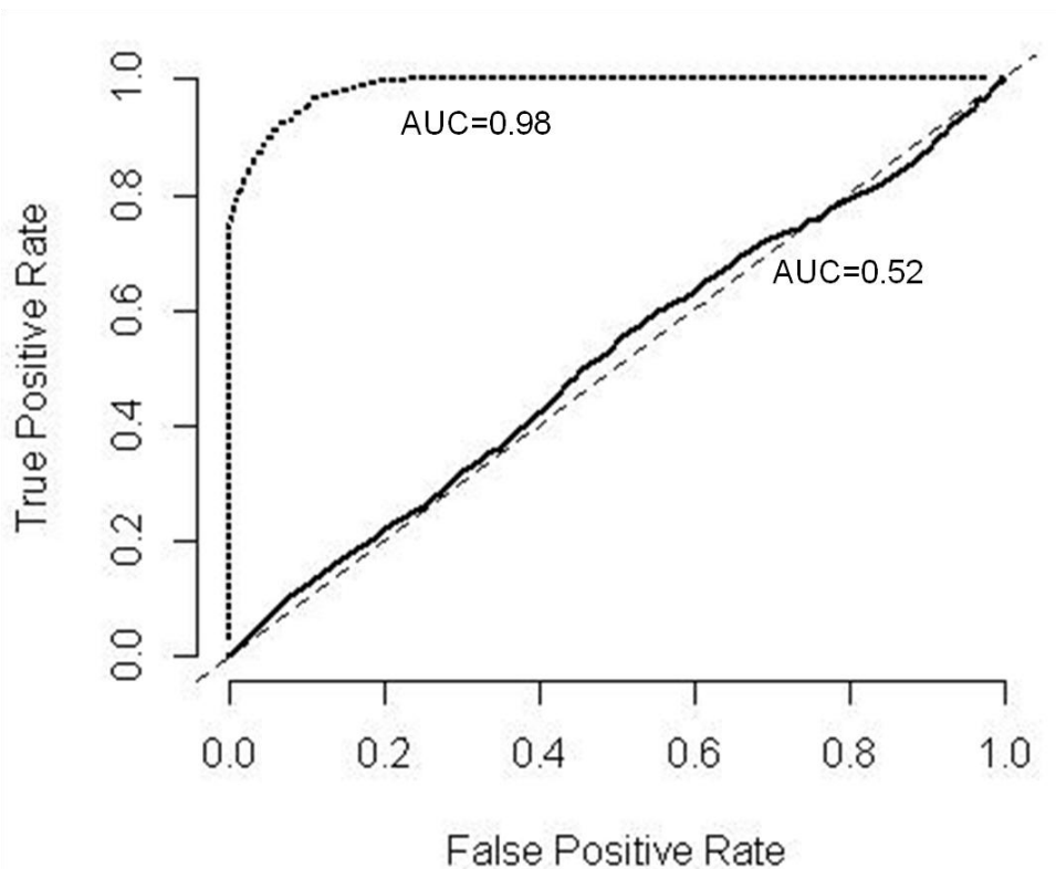
Figure 3. Two sample ROC curves for hypothetical indicators across threshold values of 0-100%. The ROC curves have an area under the curve (AUC) of 0.98 (dotted line) and 0.52 (solid line).
