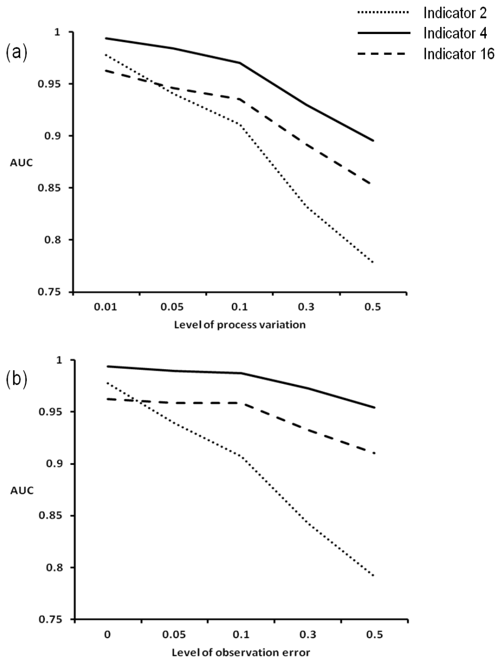
Figure 5. The area under the curve (AUC) values for selected indicators across increasing levels of (a) process variation and (b) observation error. The indicators are a high-reliability indicator based on a historical baseline at the beginning of the time series (indicator 4 [solid line]), a medium-reliability indicator based on a maximum abundance baseline (indicator 16 [dashed line]), and the commonly used IUCN indicator based on decline over the most recent three generations (indicator 2 [dotted line]).
