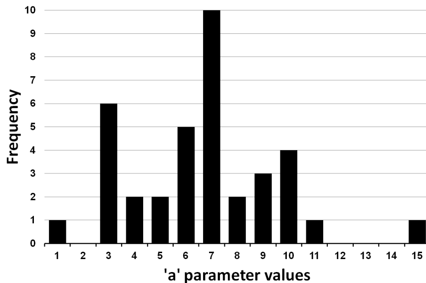
Figure A1. Frequency of 'a' parameter values derived from the \alpha parameter values from Dorner et al. (2009) data.
