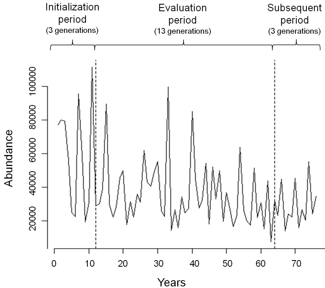
Figure 1. An example of periods in the time series output produced by the model.
