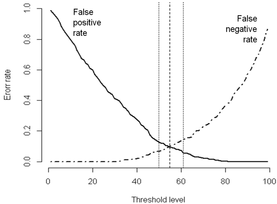
Figure 6. An example of the false positive rate (solid) and false negative rate (dot-dash) across threshold levels for classifying a population as declining ranging from 0-100% for indicator #16 for the base-case scenario with low process variation and no observation error ( \sigma_u^2=0.01 , \sigma_v^2=0 ). The black dashed vertical line indicates the threshold where both error rates are equal (i.e., the lowest rate of both error types if they are considered equally important). The dotted vertical lines indicate the lowest error rates if a false negative is considered twice as important as a false positive (left vertical dotted line, i.e., that the false negative rate must be half the false positive rate), and vice-versa (right vertical dotted line).
