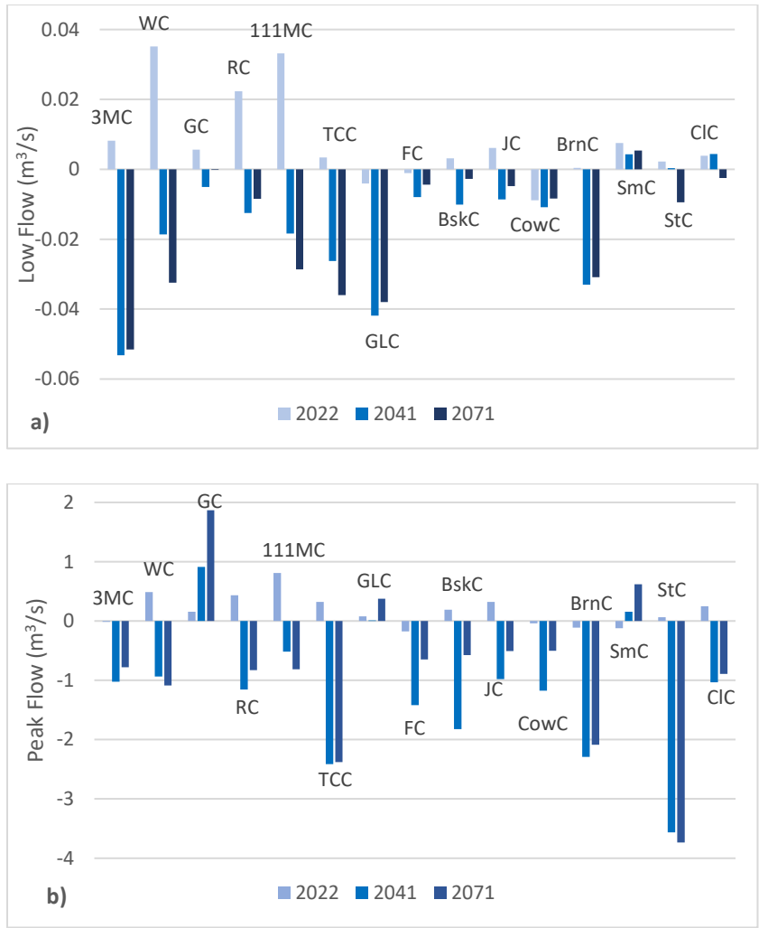
Figure 14. Bar charts of the 15 field sites showing (a) 2022 estimated low flows with climate data and 2041 and 2071 projected low flows by field site; (b) 2022 estimated peak flows with climate data and 2041 and 2071 projected peak flows by field site. Site codes shown in Section 4.7 Figure Naming Conventions.
