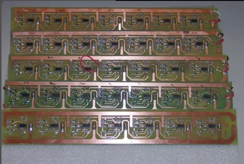
LED Boards for 49 LEDs
