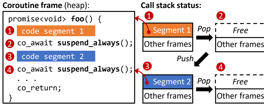
Figure 2.1: Stackless coroutine that directly uses the underlying thread’s stack. States (e.g., local variables and return value) are maintained in dynamically allocated memory.
