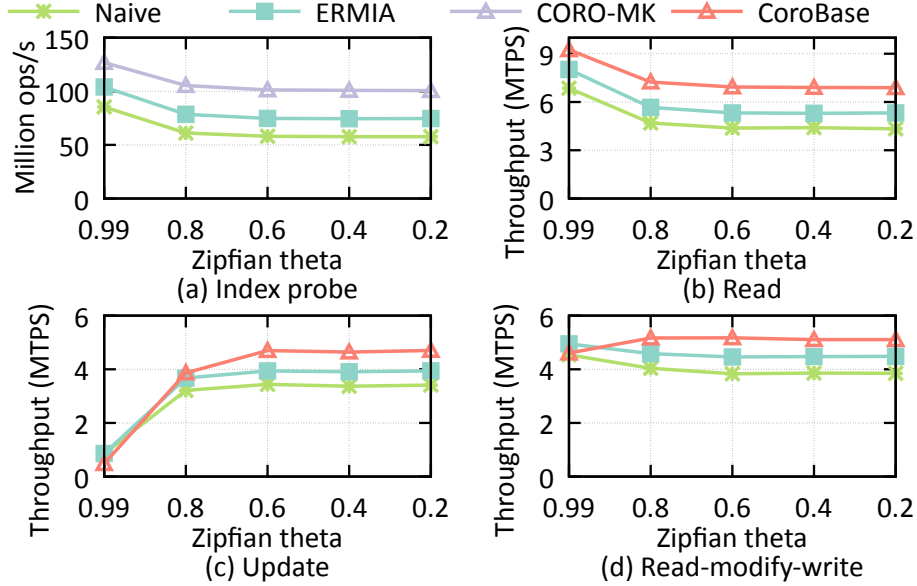
Figure 5.8: YCSB throughput with 96 hyperthreads and varying skewness (larger theta indicates more skewed access).
