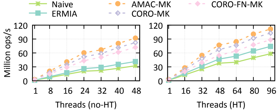
Figure 5.1: Index probing throughput with hyperthreading disabled (left) and enabled (right). Fully-nested coroutines are \sim 30\% slower than AMAC. Flattened coroutines (CORO-MK) reduce the gap to 8–10% under high concurrency.
