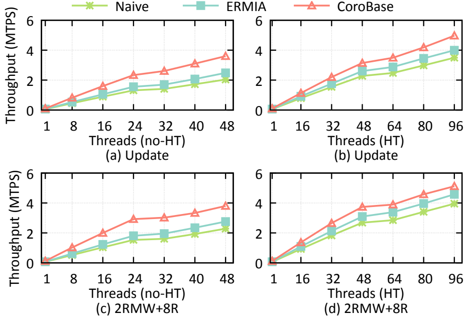
Figure 5.4: Throughput of update-only YCSB with 10 blind writes per transaction (a–b), and a mixed workload (c–d).
