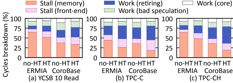
Figure 5.9: Microarchitecture analysis for YCSB, TPC-C and TPC-CH workloads. CoroBase reduces memory stall cycles under all workloads, especially the read-dominant ones.
