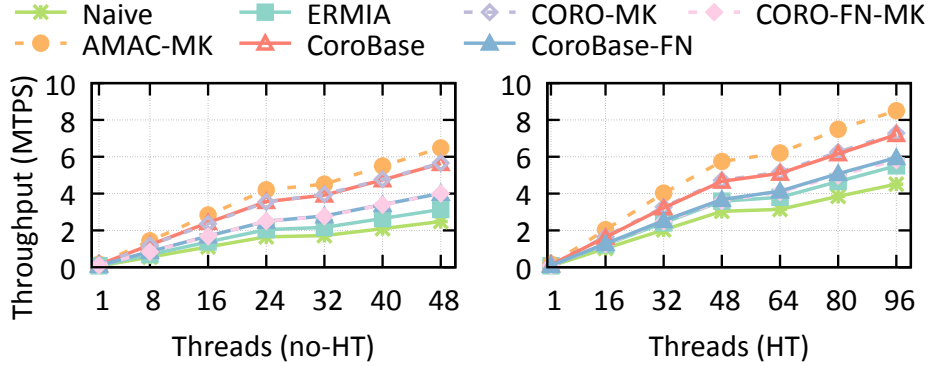
Figure 5.2: Throughput of a read-only YCSB workload (10 reads per transaction) without (left) and with (right) hyperthreading. CoroBase matches the performance of multi-key variants but without requiring application changes.
