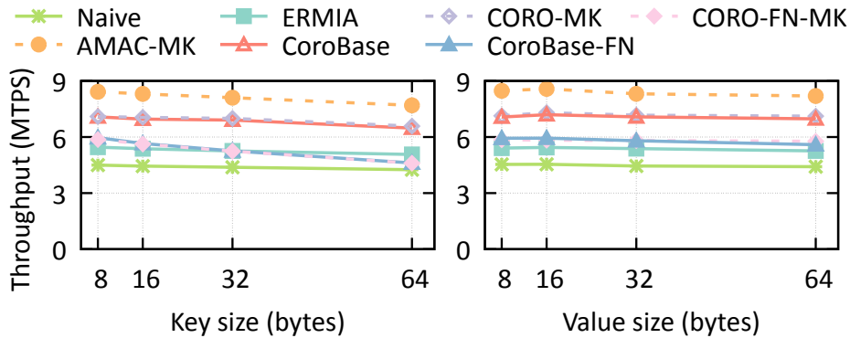
Figure 5.6: Throughput of read-only YCSB (10 reads per transaction) under varying key/-value sizes and 96 hyperthreads.
