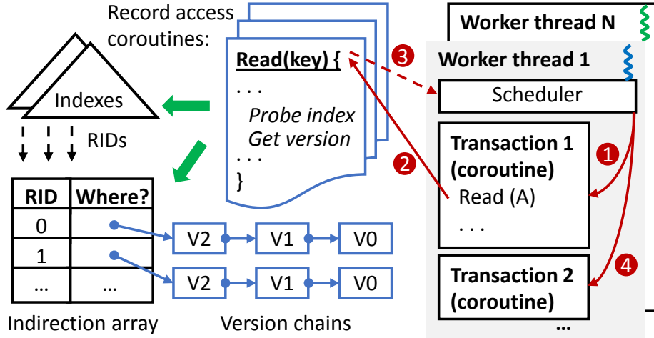
Figure 4.1: CoroBase overview. Indexes map keys to unique record IDs (RIDs). Versions are maintained by version chains. Each worker thread runs a scheduler that ❶ starts/resumes transactions (coroutines). ❷ A transaction may invoke other coroutines that implement specific operations, which may suspend but ❸ return control directly to the scheduler, which can ❹ resume a different transaction.
