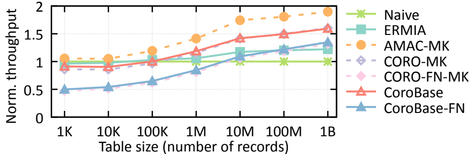
Figure 5.7: YCSB read-only (10 reads per transaction) performance normalized to Naive under 96 hyperthreads and varying table sizes.
