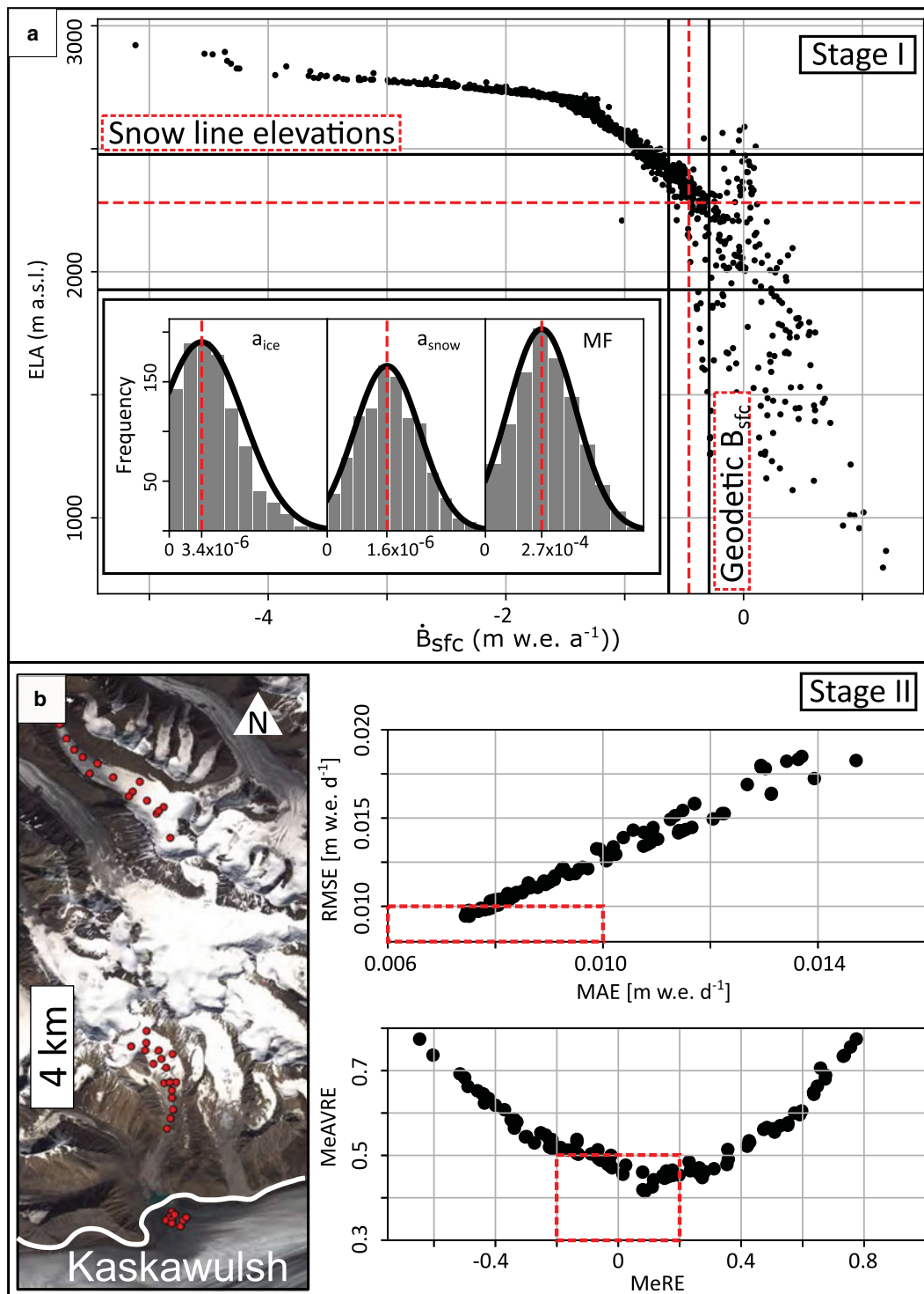
Fig. 6. Two-stage model tuning shown for debris-present simulations. The same procedure is carried out for debris-free simulations (see Supplementary material). (a) Stage 1. Modelled ELA vs glacier-wide mass balance for 2007–18 for 1000 simulations (black dots) with values of MF (m w.e. 3 \text{ h}^{-1} \text{ C}^{-1} ), a_{\text{ice}} and a_{\text{snow}} (m w.e. 3 \text{ h}^{-1} \text{ C}^{-1} \text{ m}^2 \text{ W}^{-1} ) randomly selected from normal distributions truncated at zero (inset). Observational targets (red-dashed lines) are shown for ELA and glacier-wide mass balance. Simulations falling within the observational uncertainty (black lines) proceeded to Stage 2. (b) Stage 2. RMSE vs MAE (top) and median of the absolute value of the relative error (MeAVRE) vs the median of the relative error (MeRE) between modelled and measured net ablation (bottom) at 44 locations (map at left). Twelve simulations falling within both red-dashed rectangles pass Stage 2.
