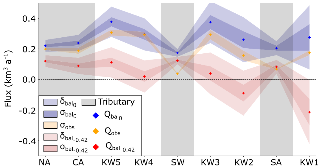
Fig. 10. Comparison of observed and balance fluxes arranged according to position of flux gate (tributaries shaded in grey). See Figure 8 for flux-gate locations. Observed fluxes ( Q_{\text{obs}} , yellow) are shown with standard deviations arising only from glacier-bed interpretation (see Q_{\text{ref}} in Table 3). Balance fluxes are shown for \bar{B}_{\text{sfc}} = 0 ( Q_{\text{bal}_0} , blue) and \bar{B}_{\text{sfc}} = -0.42 m w.e. ( Q_{\text{bal}_{-0.42}} , red). Dark red/blue shading is standard deviation of balance fluxes for the 12 simulations that satisfy both stages of model tuning for debris-present case. Light red/blue shading is the uncertainty for each balance flux determined from the uncertainties on model accumulation and melt rates. Shading is continuous between flux gates only to assist in visual interpretation; not all flux gates are connected as suggested by shading.
