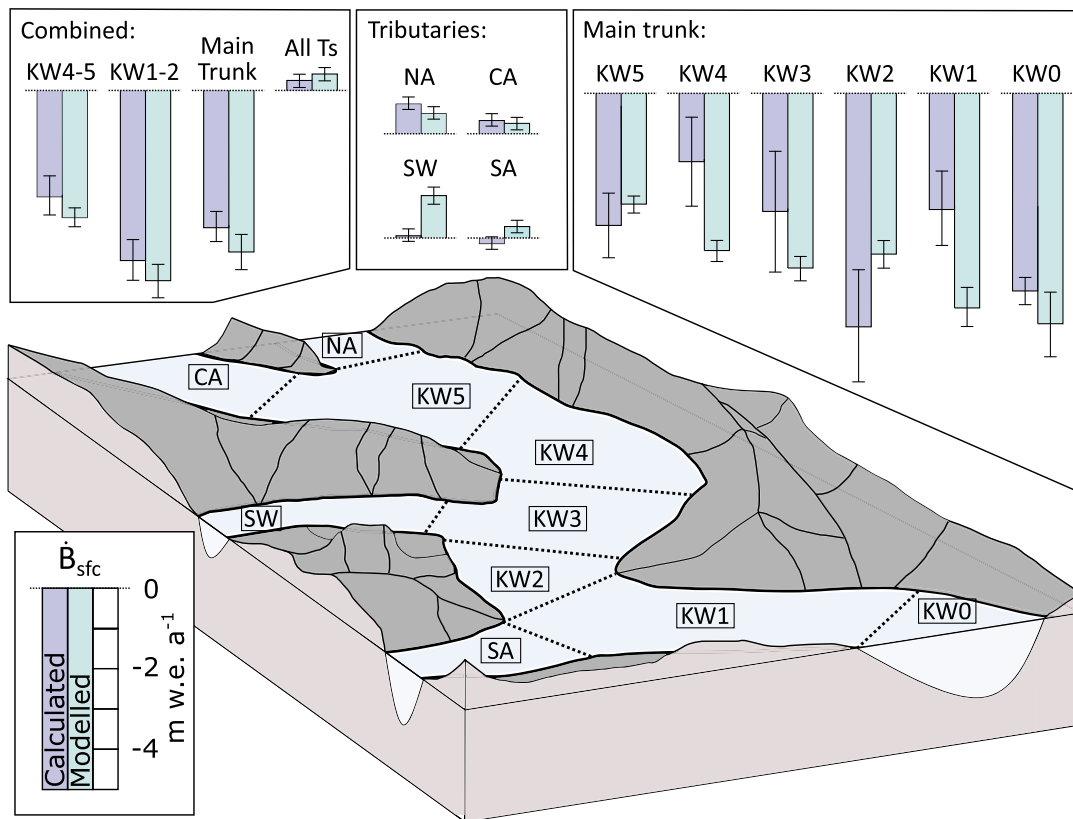
Fig. 9. Comparison of calculated ( \dot{B}_{cal} , light purple) and modelled ( \dot{B}_{mod} , light blue) mass balance, with associated uncertainties, for each section of the glacier. Sections are labelled according to their downstream flux gates. Also shown are four combined sections: KW4 and KW5 ('KW4-5'); KW1 and KW2 ('KW1-2'); KW0 through KW5 ('Main trunk'); and NA, CA, SW, SA ('All Ts' for all tributaries).
