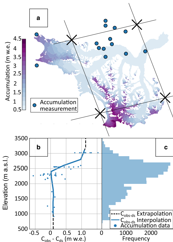
Fig. 5. Precipitation downscaling and accumulation bias correction. (a) Mean annual accumulation field for 2007–18 following downscaling of NARR daily surface precipitation and bias correction of accumulation. Locations of four NARR grid nodes (black crosses) and snow depth/density measurements (blue circles) are shown. Eight additional snow-measurement locations are not shown due to scale. (b) Interpolated (solid blue line) and extrapolated (dashed black line) elevation-dependent values of difference between measured and downscaled accumulation ( C_{\text{obs}} - C_{\text{ds}} ), along with values of C_{\text{obs}} - C_{\text{ds}} at measurement locations (blue dots). (c) Hypsometry of Kaskawulsh Glacier, with frequency of 200 m × 200 m gridcells in each bin.
