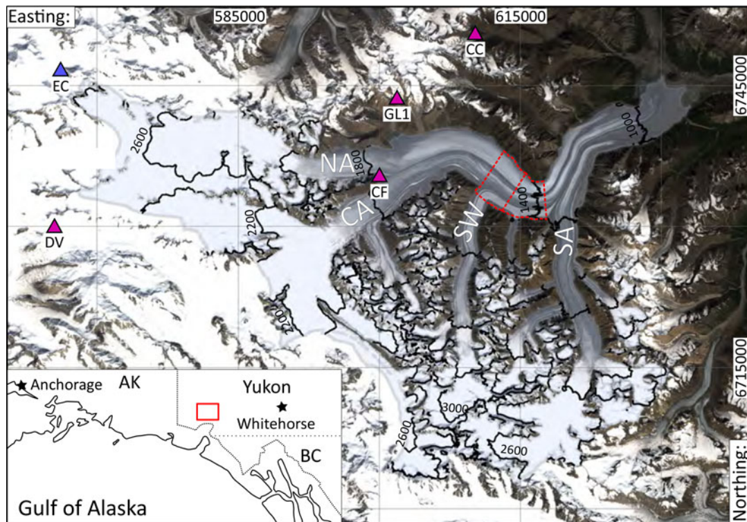
Fig. 1. Study area (red box, inset) and overview of Kaskawulsh Glacier. Kaskawulsh Glacier highlighted in blue (regions where surface is darker are debris-covered), with major tributaries labelled: North Arm (NA), Central Arm (CA), Stairway Glacier (SW), South Arm (SA). Also shown are locations of automatic weather stations (magenta triangles) and Eclipse Icefield site with multi-annual accumulation data (blue triangle) (Kelsey and others, 2012). Red-dashed lines indicate position of balance terminus position, referred to in the 'Analysis and interpretation' section. Black contours are m a.s.l. and coordinates are UTM Zone 7 North. Background image: Copernicus Sentinel data 2017. Retrieved from Copernicus Open Access Hub 01/11/17.
