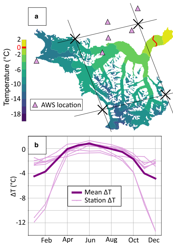
Fig. 4. Temperature downscaling and bias correction. (a) Mean 2 m air temperature field for 2007–18 following downscaling and bias correction of NARR data. Locations of four NARR grid nodes (black crosses) and six AWS (purple triangles) are shown. Environment Canada AWS at Burwash Landing (UTM: 604700 E, 6805731 N) and Haines junction (UTM: 698045 E, 6704555 N) are not shown due to scale. (b) Monthly values of \Delta T for each AWS (fine pink lines) along with mean monthly \Delta T used for bias correction of downscaled temperatures (bold purple line). Anomalously low values of \Delta T are from Burwash Landing and Haines Junction, both a minimum of \sim 60 km from the Kaskawulsh Glacier.
