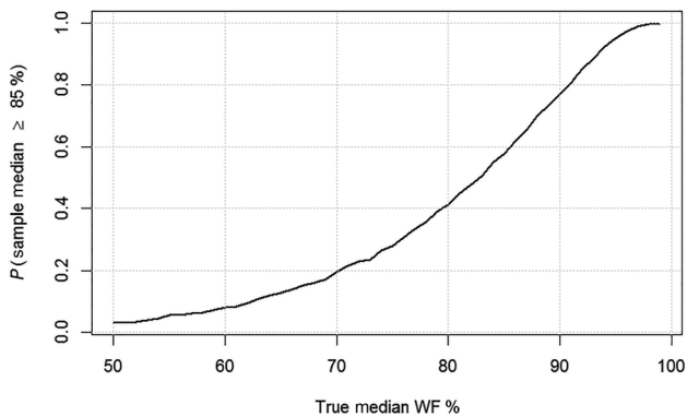
FIG. 5 Estimated probability that a laboratory produces data with a median WF% of at least 85 %, given different true median values.
