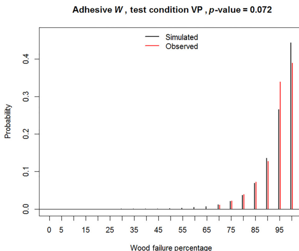
FIG. 4 Comparison of observed and model-simulated marginal distributions for a case showing more recordings of 95 % and fewer than 100 % expected under the model.
